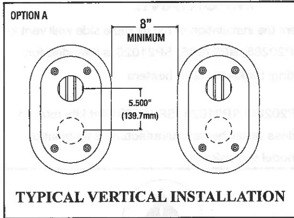
FIGURE 1 VENT KIT INSTALLATION OPTIONS
