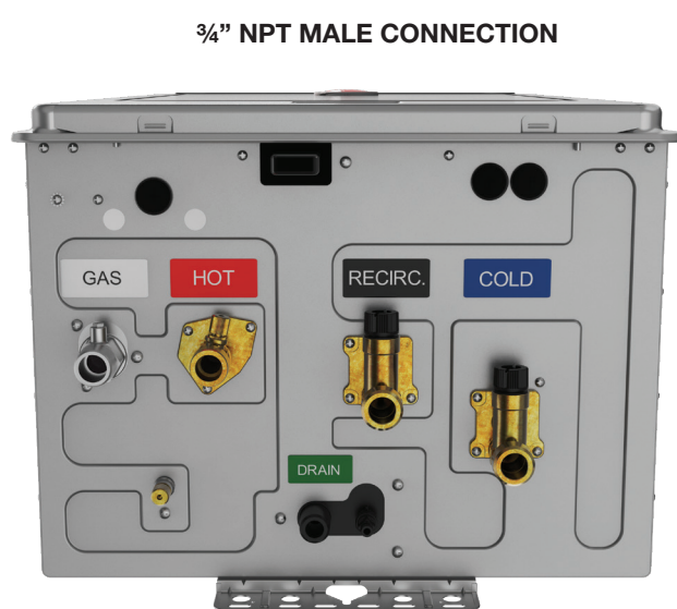
3/4" NPT MALE CONNECTION
